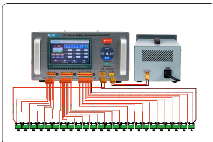
HTB-J24S25AC equalizer XT60 interface (Adaptable to other brands of equalizers on the market)
