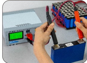
Measure the lithium iron phosphate battery: IR:0.273mΩ, V:3.737V.
