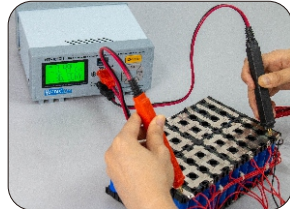
Measure the 20S 48V 18650 battery pack: IR:0.4942Ω, V:36.906V.
